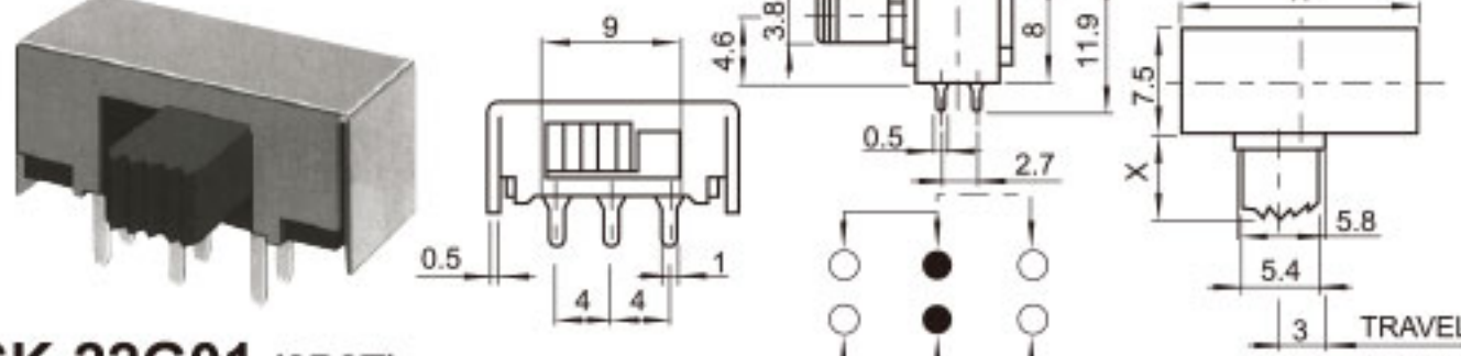
SK-22G01 (2P2T)
