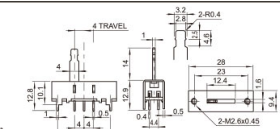
SS-12G04A (1P2T)
