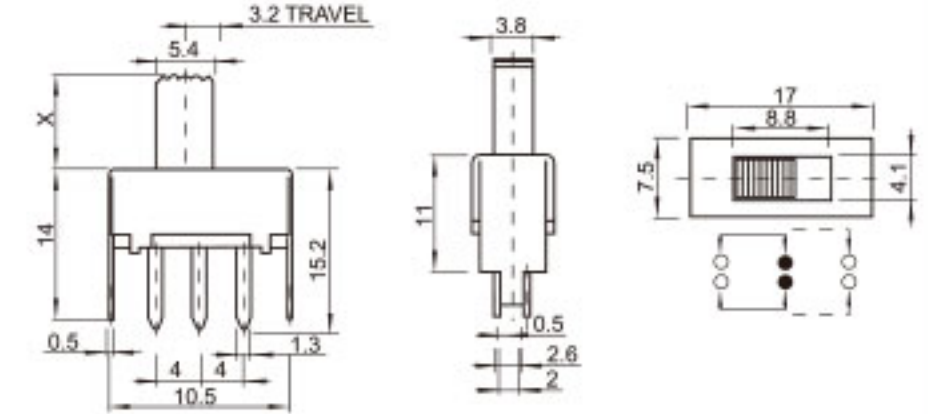
SS-22G50 (2P2T)
