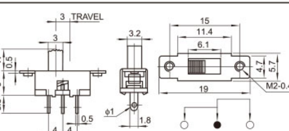
SS-12F77 (1P2T)
