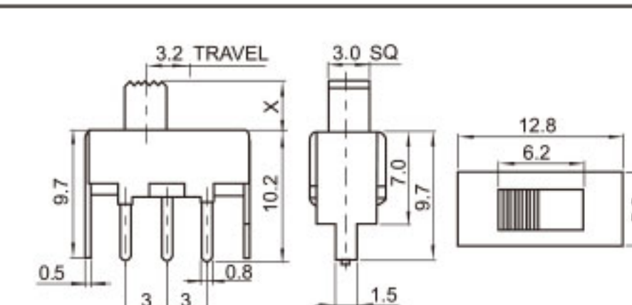
SS-12F47 (1P2T)
