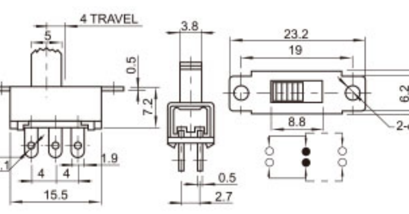
SS-22G32 (2P2T)
