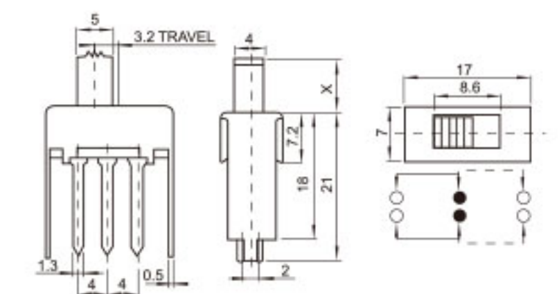
SS-22G20 (2P2T)
