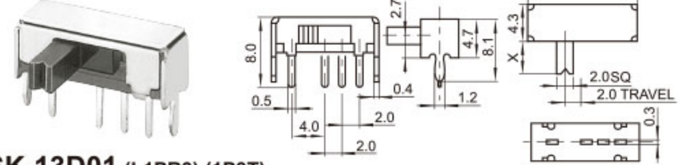
SK-13D01 (L1PR3) (1P3T)
