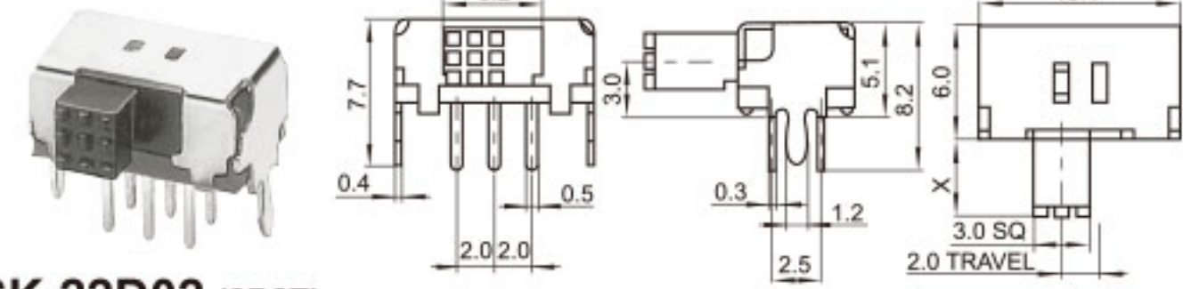
SK-22D02 (2P2T)
