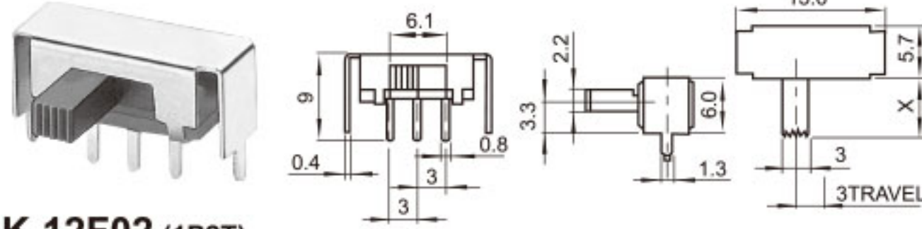
SK-12F02 (1P2T)
