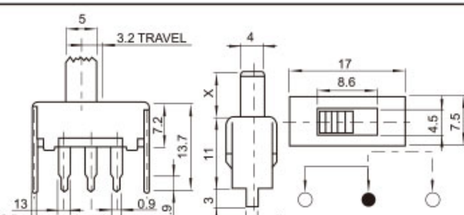
SS-12G04 (1P2T)
