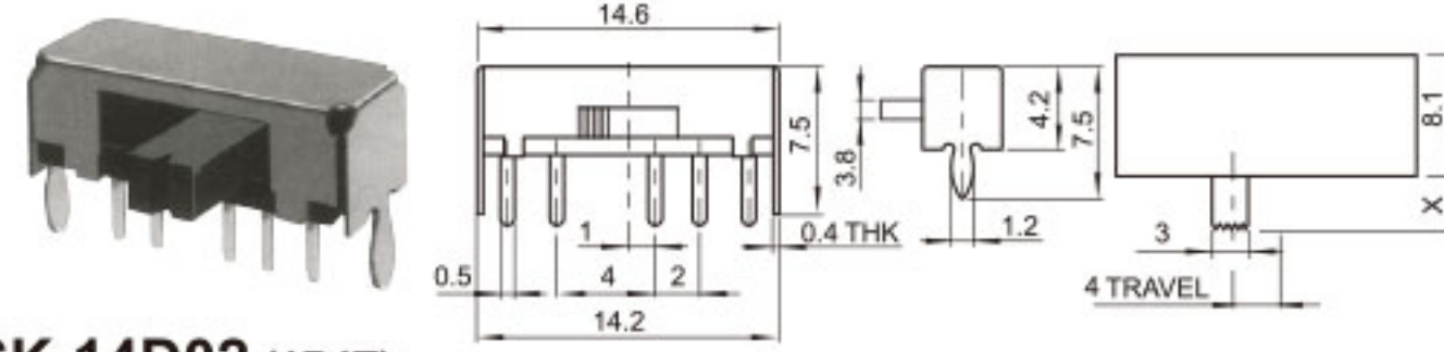
SK-14D02 (1P4T)
