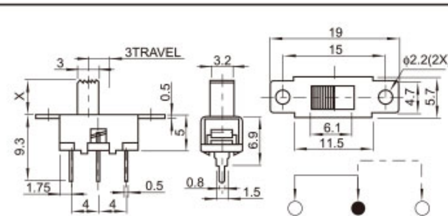
SS-12F75 (1P2T)
