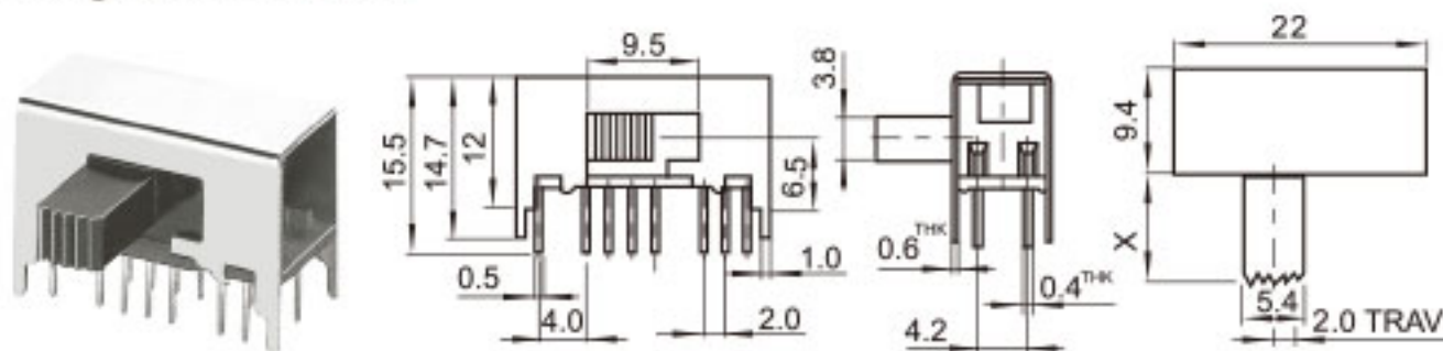
SS-43D03 (L1R3) (4P3T)
