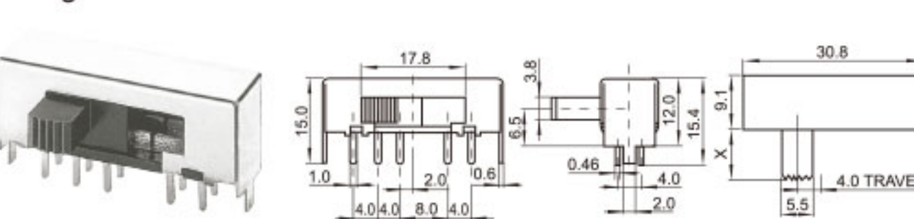
SS-24H02 (2P4T)
