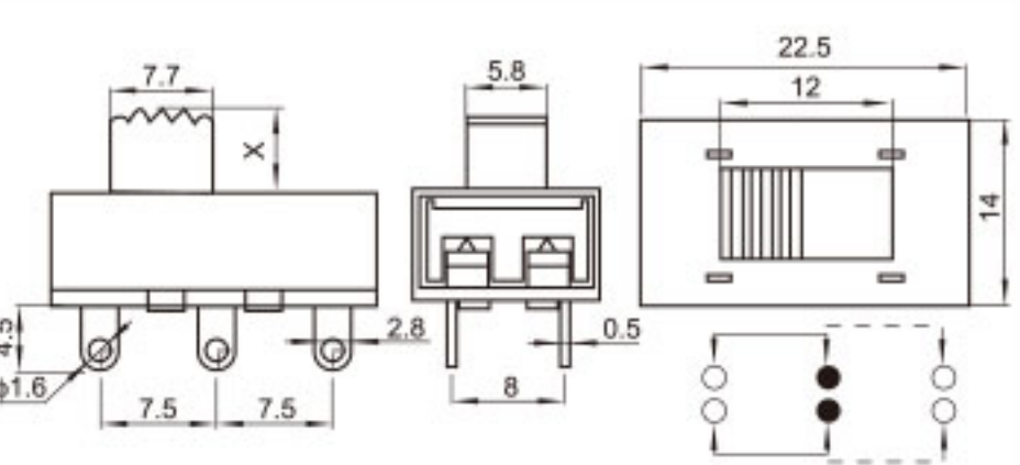
SS-22H01 (2P2T)
