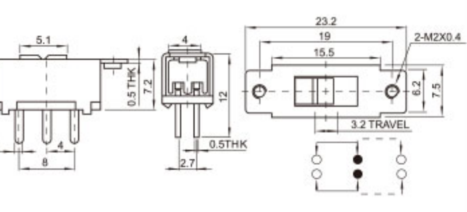
SS-22G96 (2P2T)
