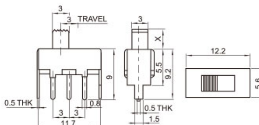
SS-12F45 (1P2T)
