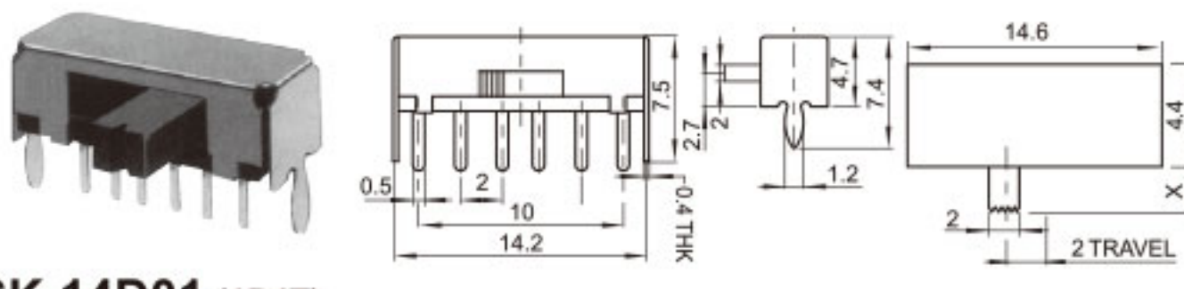
SK-14D01 (1P4T)
