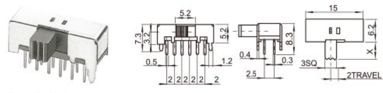
SS-42D01 (4P2T)
