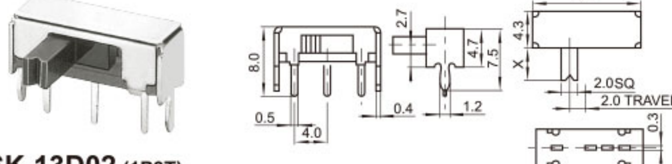
SK-13D02 (1P3T)
