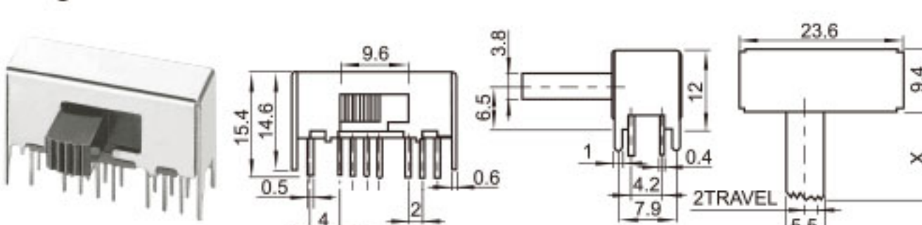
SS-43D01 (4P3T)
