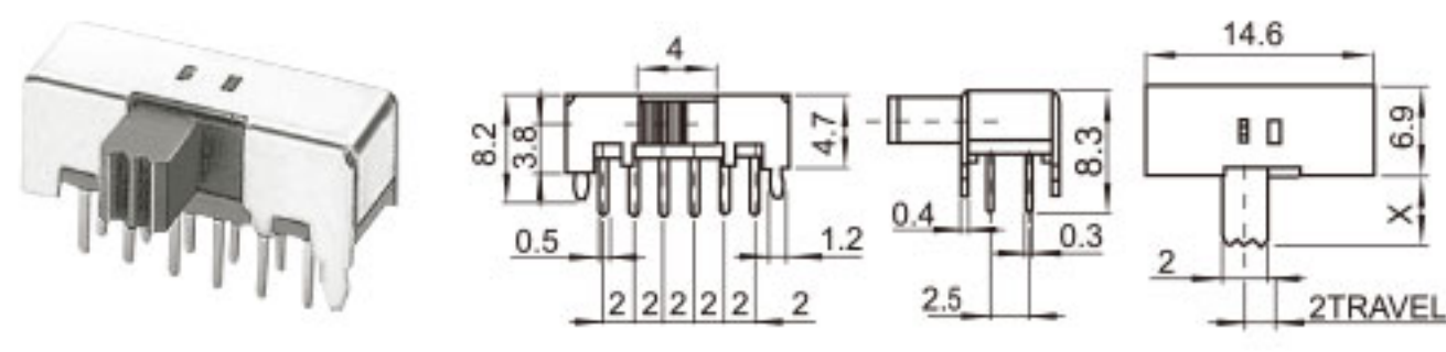
SS-42D02 (4P2T)
