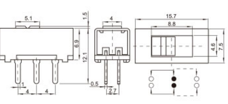
SS-22G93 (2P2T)
