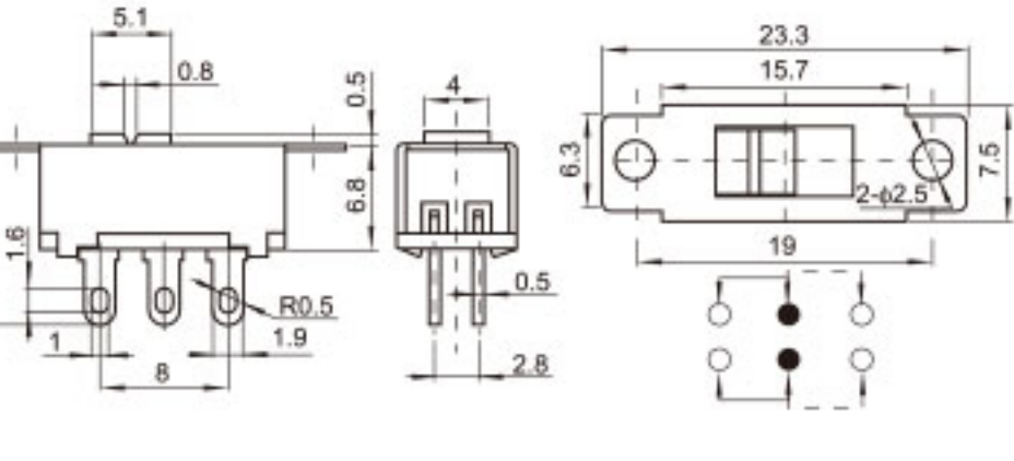
SS-22G95 (2P2T)
