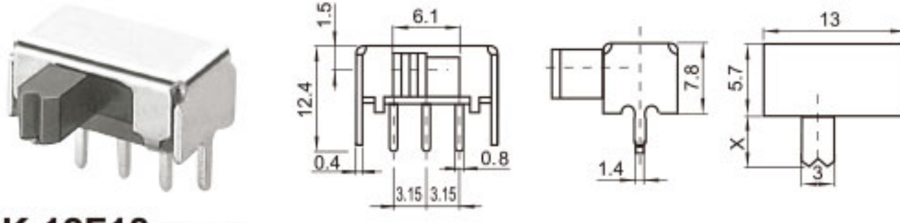
SK-12F18 (1P2T)
