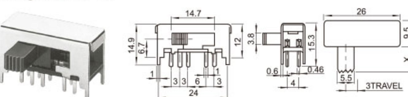
SS-24F01 (L3R2) (2P4T)
