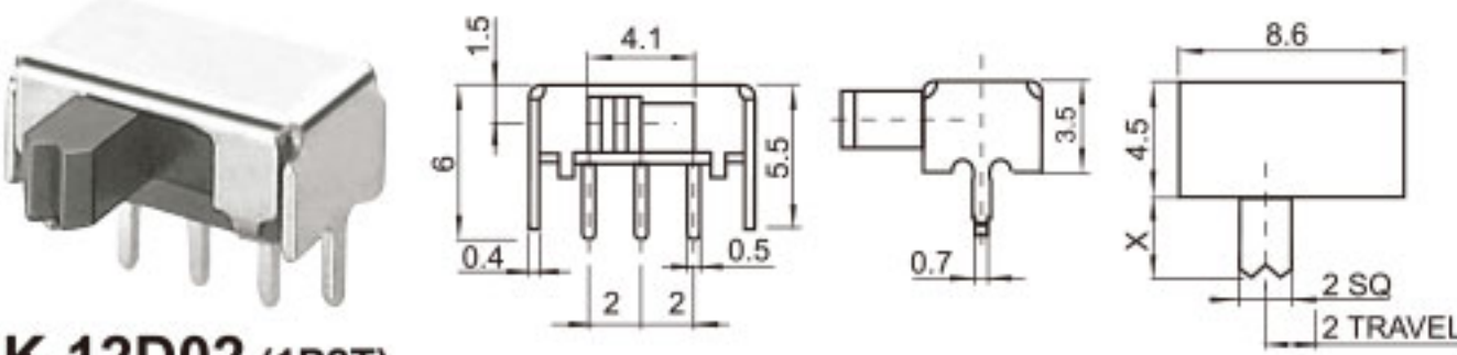
SK-12D02 (1P2T)
