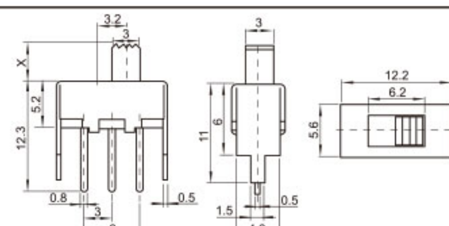
SS-12F68 (1P2T)
