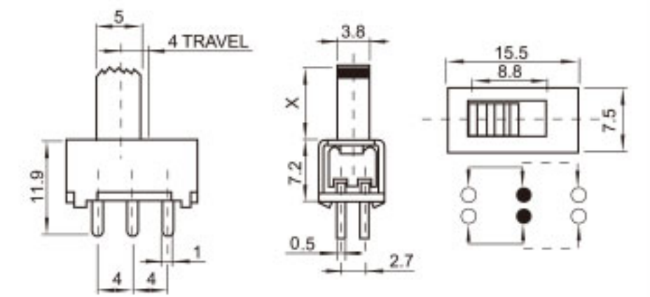
SS-22G91 (2P2T)
