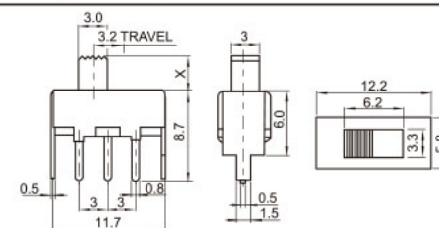
SS-12F46 (1P2T)
