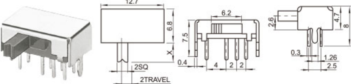
SK-23D07 (L1R3) (2P3T)
