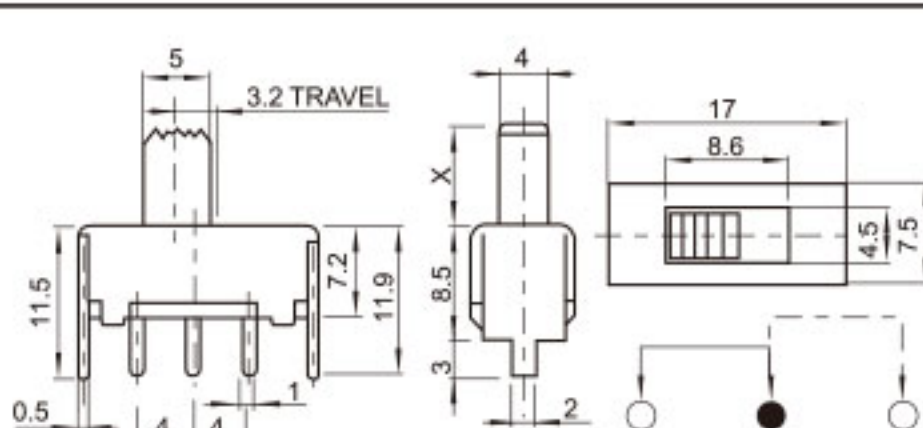
SS-12G02 (1P2T)
