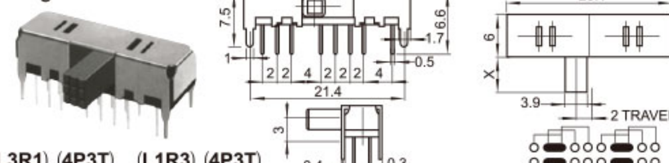
(L3R1) (4P3T) (L1R3) (4P3T) SS-43D09 SK-43D10
