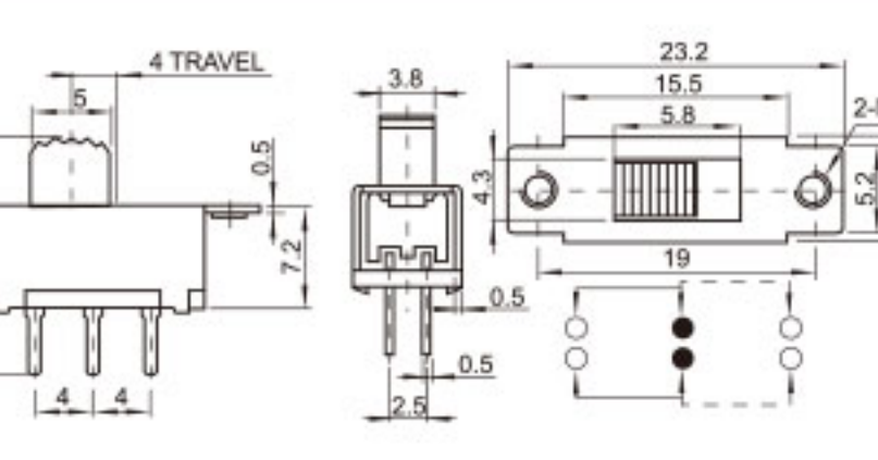
SS-22G28 (2P2T)
