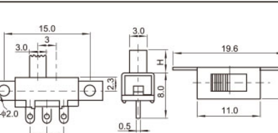
SS-12F55 (1P2T)
