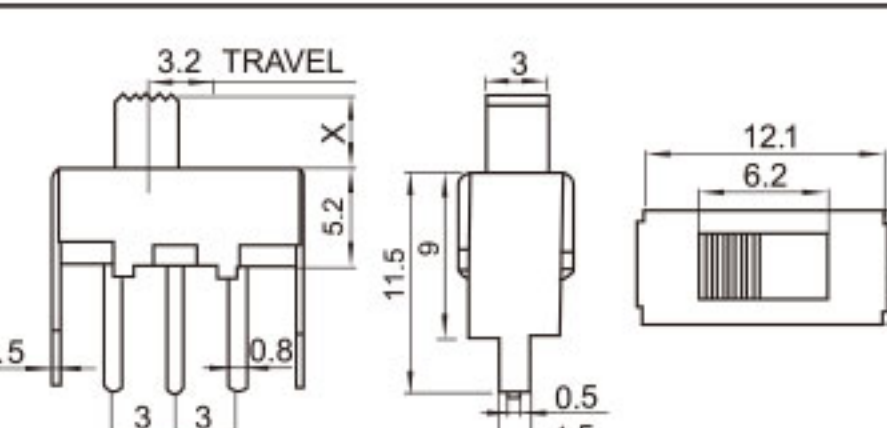
SS-12F49 (1P2T)
