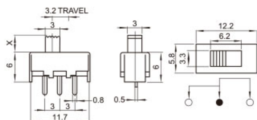
SS-12F68 (1P2T)
