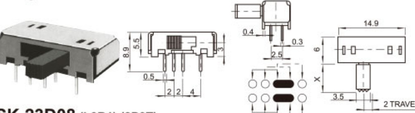
SK-23D08 (L3R1) (2P3T)
