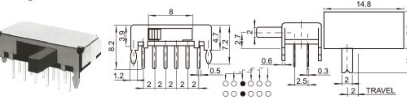
SK-24D02 (2P4T)
