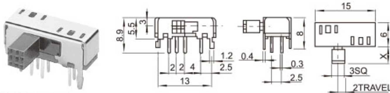
SK-23D06 (L3R1) (2P3T)
