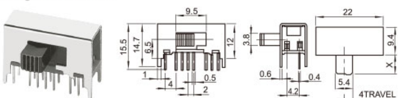
SS-42H03 (L1R3) (4P2T)
