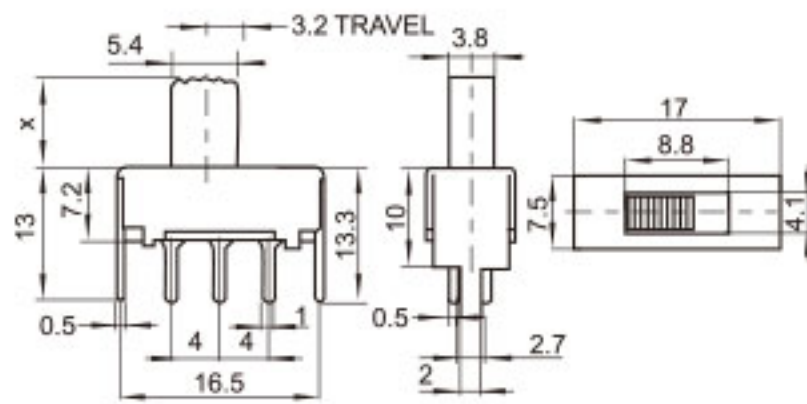
SS-22G10 (2P2T)
