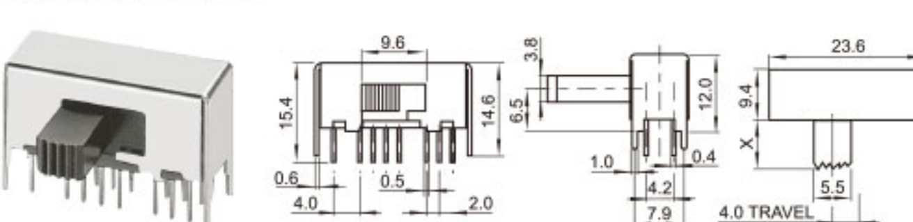
SS-42H01 (4P2T)
