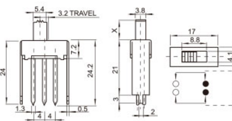
SS-22G24 (2P2T)
