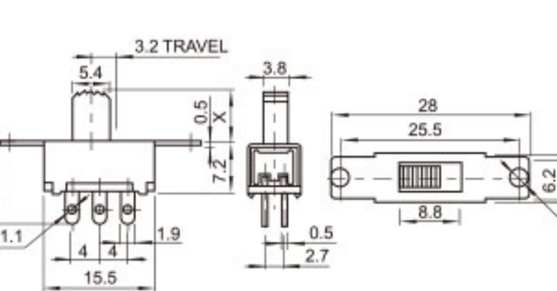
SS-22G26 (2P2T)
