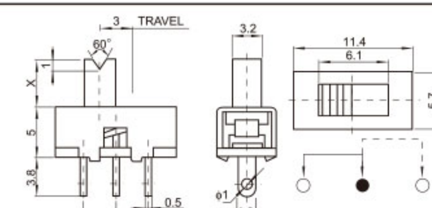
SS-12F51 (1P2T)
