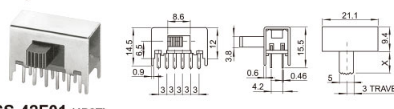
SS-42F01 (4P2T)
