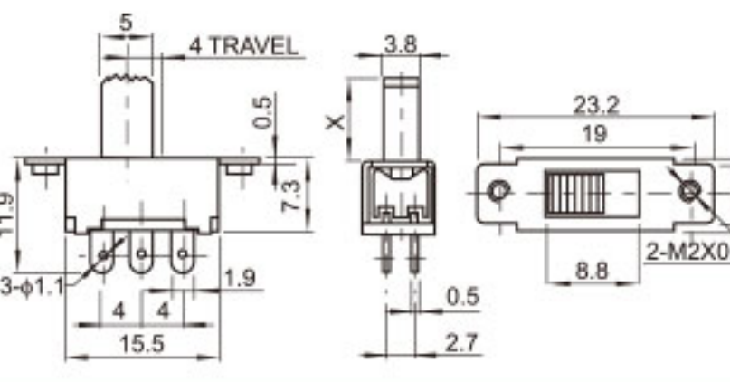
SS-22G25 (2P2T)
